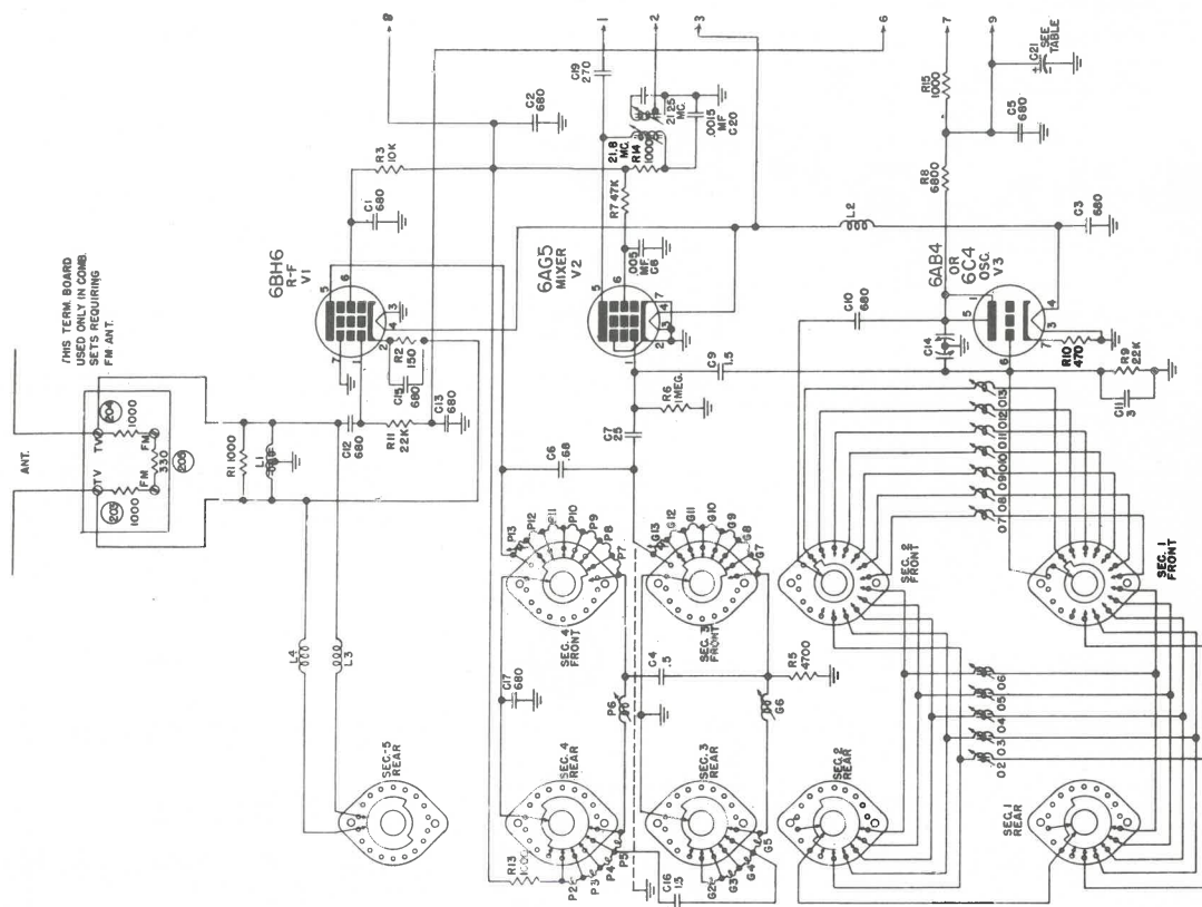
MAGNAVOX RF TUNER CHASSIS CT232, CT239
